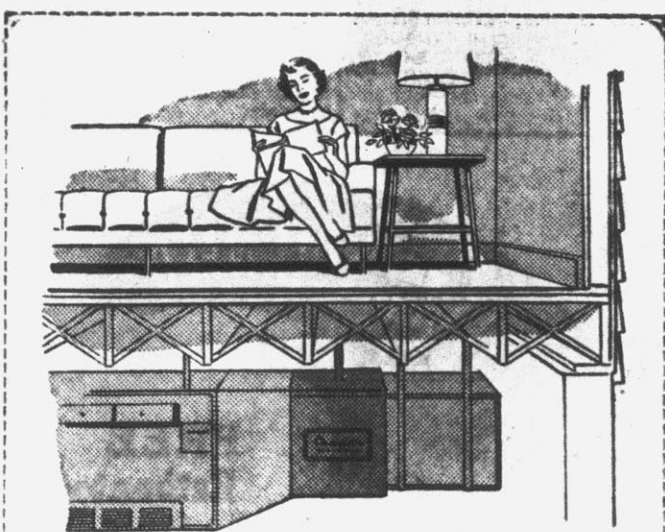
Carrier Conversion Weathermakers inexpensively add cooling to any warm air furnace, use fan, filter and ducts of your present system. Cooling sections fit horizontal (illustrated) and vertical furnaces. Refrigeration sections locate outdoors.
