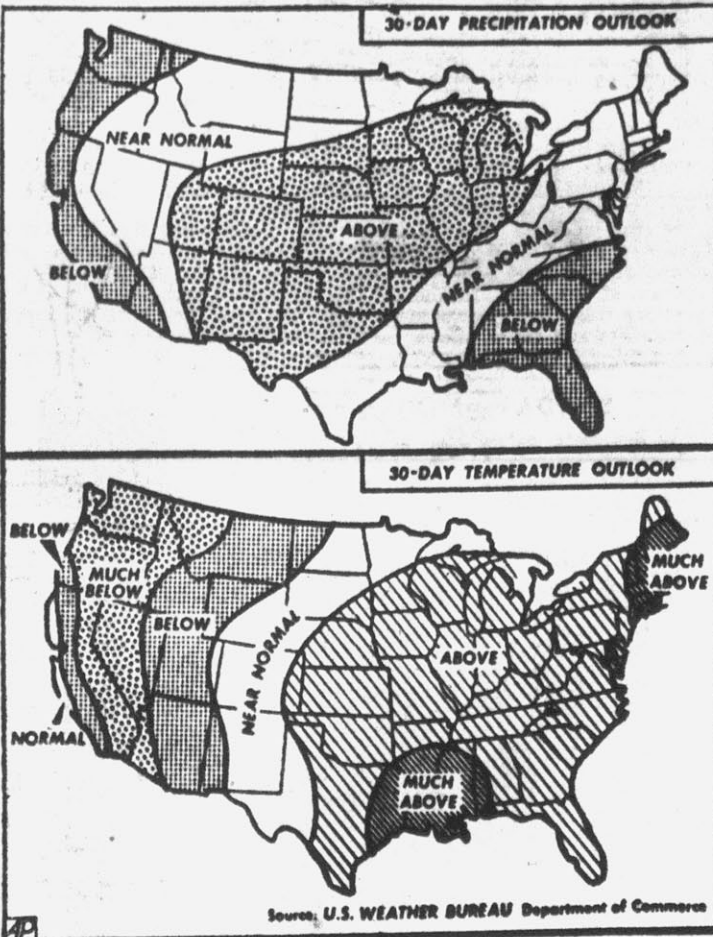
WEATHER FORECAST—These maps, based on those supplied by the U. S. Weather Bureau, forecast the probable rainfall and temperatures for the next 30 days. (AP Wirephoto Map)
