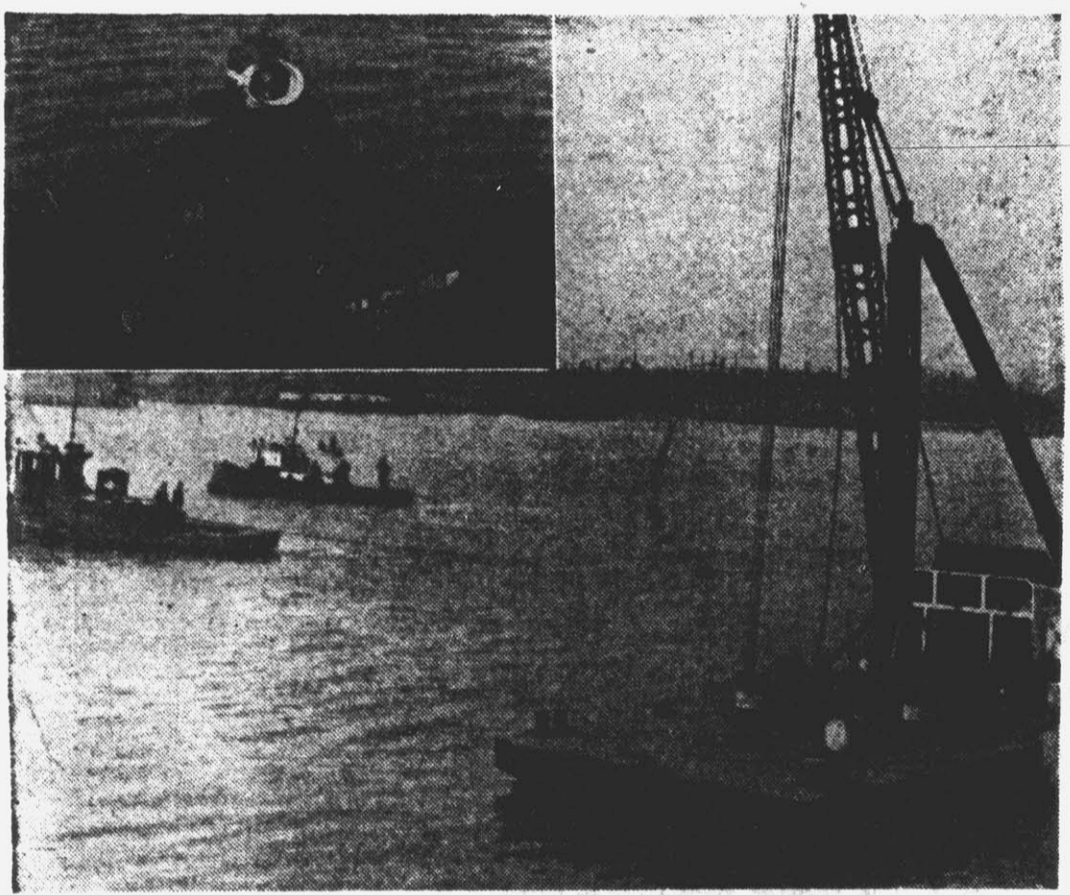
CP&L CABLES GO UNDER RIVER—To bring more electricity to Wilmington from its big, new Louis V. Sutton plant, Carolina Power & Light Company is laying submarine cables across the Cape Fear River. Here, two tugs buck the tide to straighten the tubing before it is lowered into a trench dredged in the river bed. Empty oil drums support the weight. Inset shows Bill Crane, frogman who explores the murky depths to inspect the job. The project, unique in North Carolina, is due to be completed next month.
