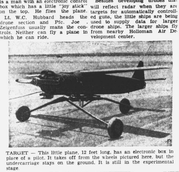
TARGET — This little plane, 12 feet long, has an electronic box in place of a pilot. It takes off from the wheels pictured here, but the undercarriage stays on the ground. It is still in the experimental stage.
