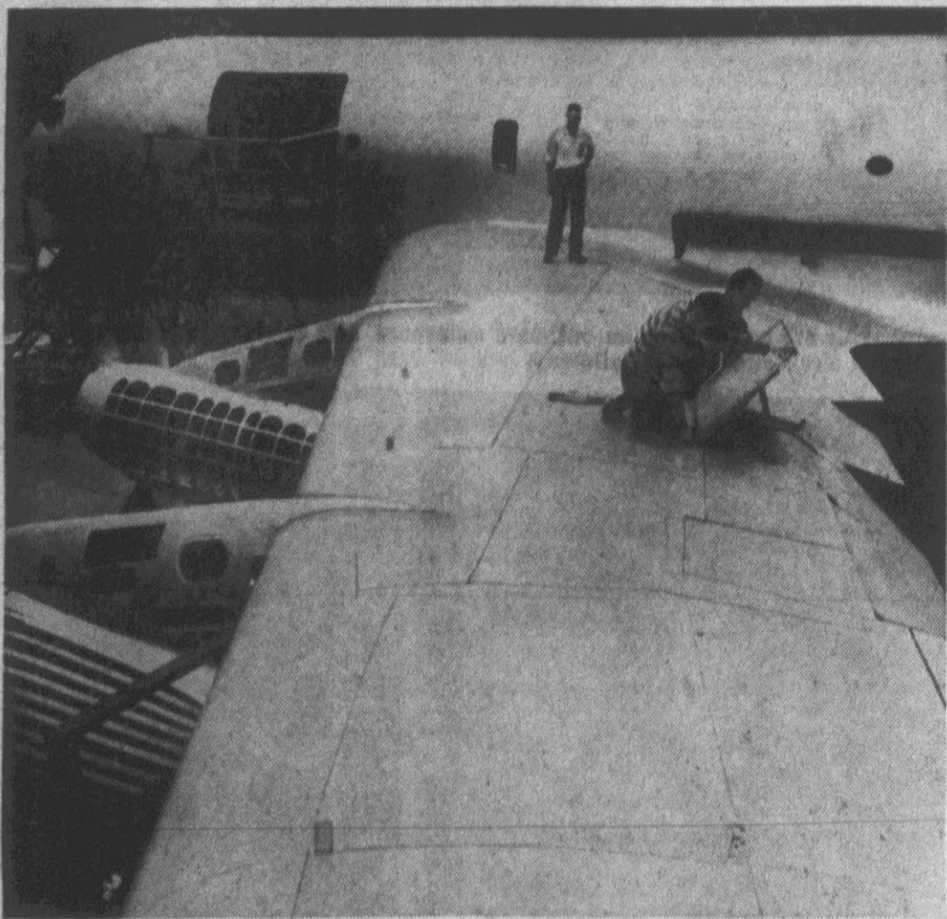
1. The 707 mock-up: Exact replica of the jet stratotanker-stratoliner built of wood as test bed for various installations and procedures used in building plane at Renton, Wash.
