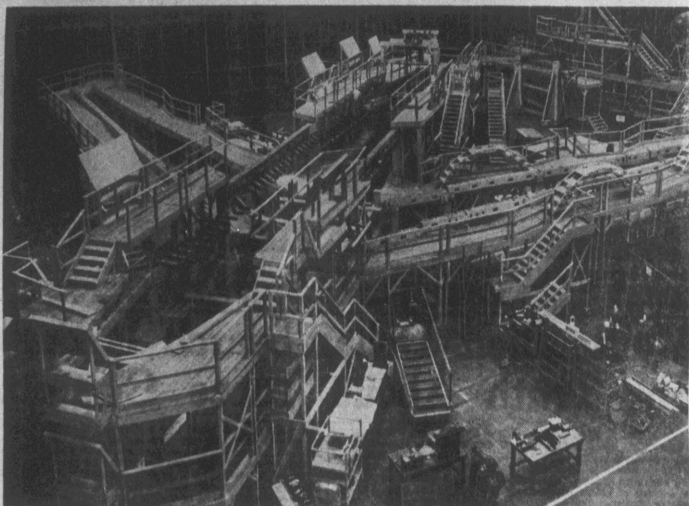
2. Wooden jig in which the Boeing 707 was built lies empty just before start of construction on actual airplane.
