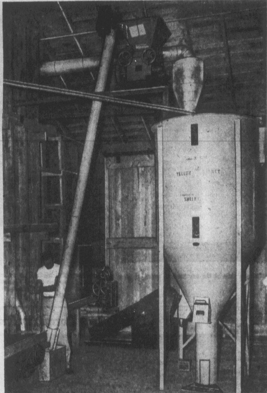
Famer Stamy looks at grain that goes into hammer mill and crimper, top, that drop corn and small grain into 1½ ton mixer, right. Automatic conveyor, left, measures small grain out of wooden bins and bazooka-type elevator takes it up to mixer.
