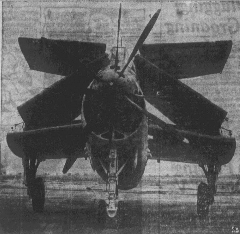
FOLDED UP FOR THE DAY — Britain's newest submarine-killer, the Fairey Gannet, taxis in with wings folded after demonstration at England's Manchester airport.
