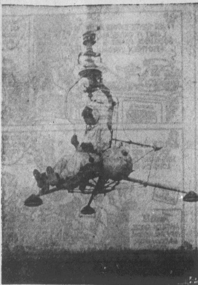
ONE-MAN WINDMILL—This may look like something out of the Wright brothers' era, but it's brand new. The Kellett KH-15 one-man helicopter, a Navy rocket-powered craft designed for research into gyro-stabilizing controls for helicopters, takes to the air at Camden, N. J. The fresh-air windmill has new controls to provide greater stability for copters. (U. S. Navy Photo via AP Wirephoto)
