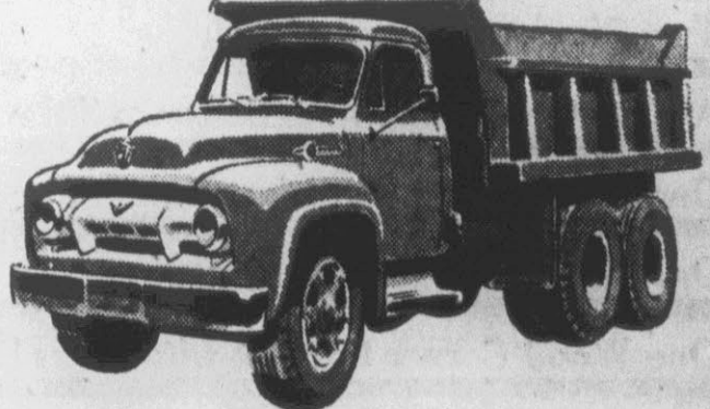
New Power Steering standard at no extra cost on new tandem-axle Ford T-800. GVW 40,000 lbs. GCW 60,000 lbs. 4 wheelbases. Overhead-valve 170-h.p. V-8 engine.
