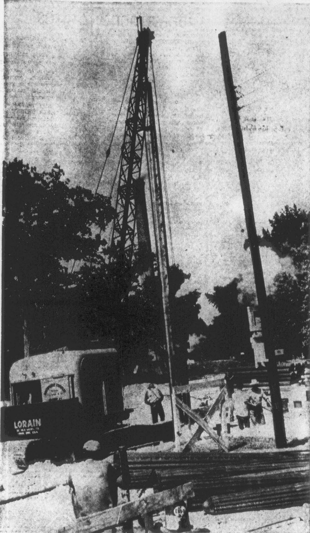
Above, a pile-driving machine sinks one of some 350 pilings which will serve as a foundation for the new men's dormitory now being constructed at East Carolina College. The metal pipes are sunk to a depth of 15 to 17 feet and will later be filled with concrete to support the building in Pitt County's sandy soil. The dormitory will face Tenth Street. (Reflector Photo by Alvin Taylor)
