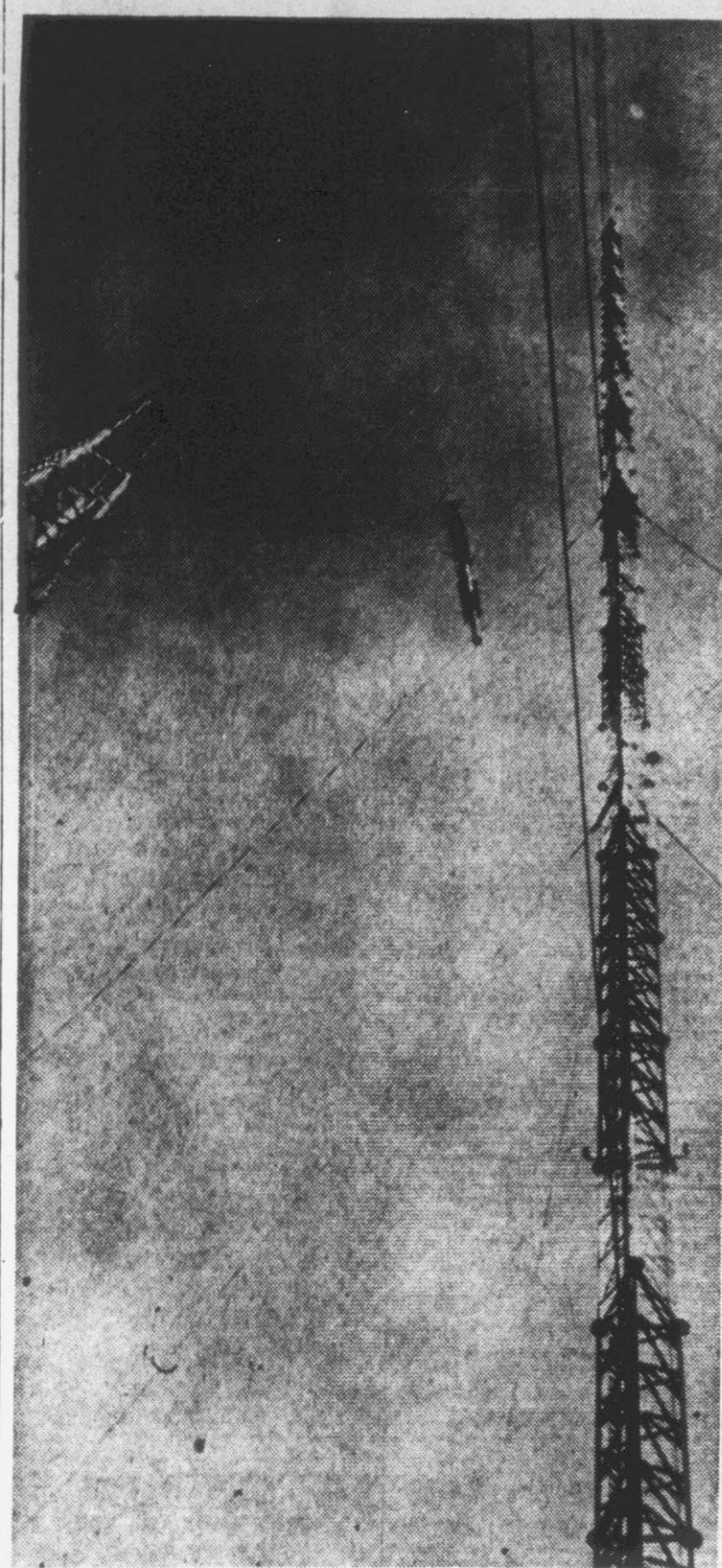
SHIFTING TO NEW TOWER —The 75-foot antenna of WNCT-TV in Greenville is shown suspended in mid-air about 400 feet above the ground as workmen moved it to the new tower. Workmen are putting final touches to the installation of the antenna on the new 800 foot tower of the station. (Photo by C. L. Perkins Jr.)
