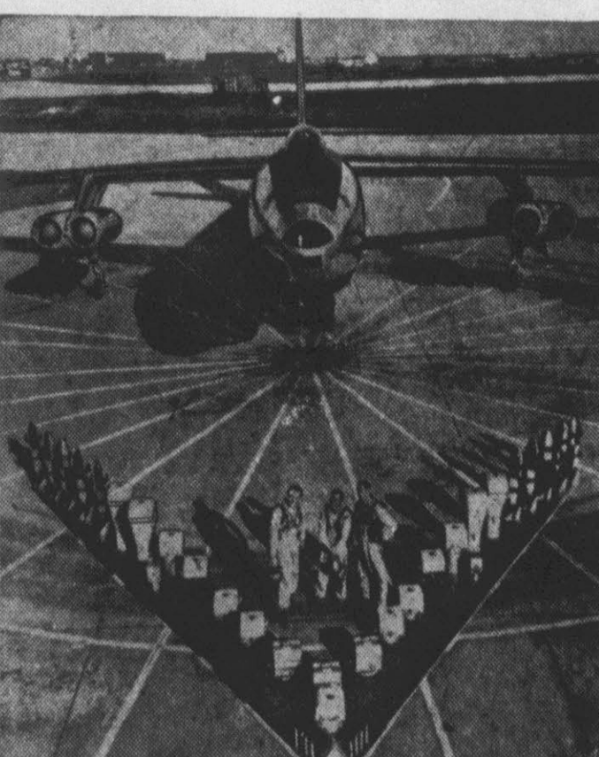
SNOOPER DELUXE—Pilot, copilot and photographer-navigator of Boeing RB47E stand amid equipment for newest photo-reconnaissance plane to go into service with the U. S. Strategic Air Command. Equipment includes 16 cameras, any seven of which may be carried at one time, depending on mission. Cylindrical objects in foreground are cartridge flares, while those at tips of the V are flash bombs. Remainder consists of 16 cameras and two photocell-operated shutter tripping units.
