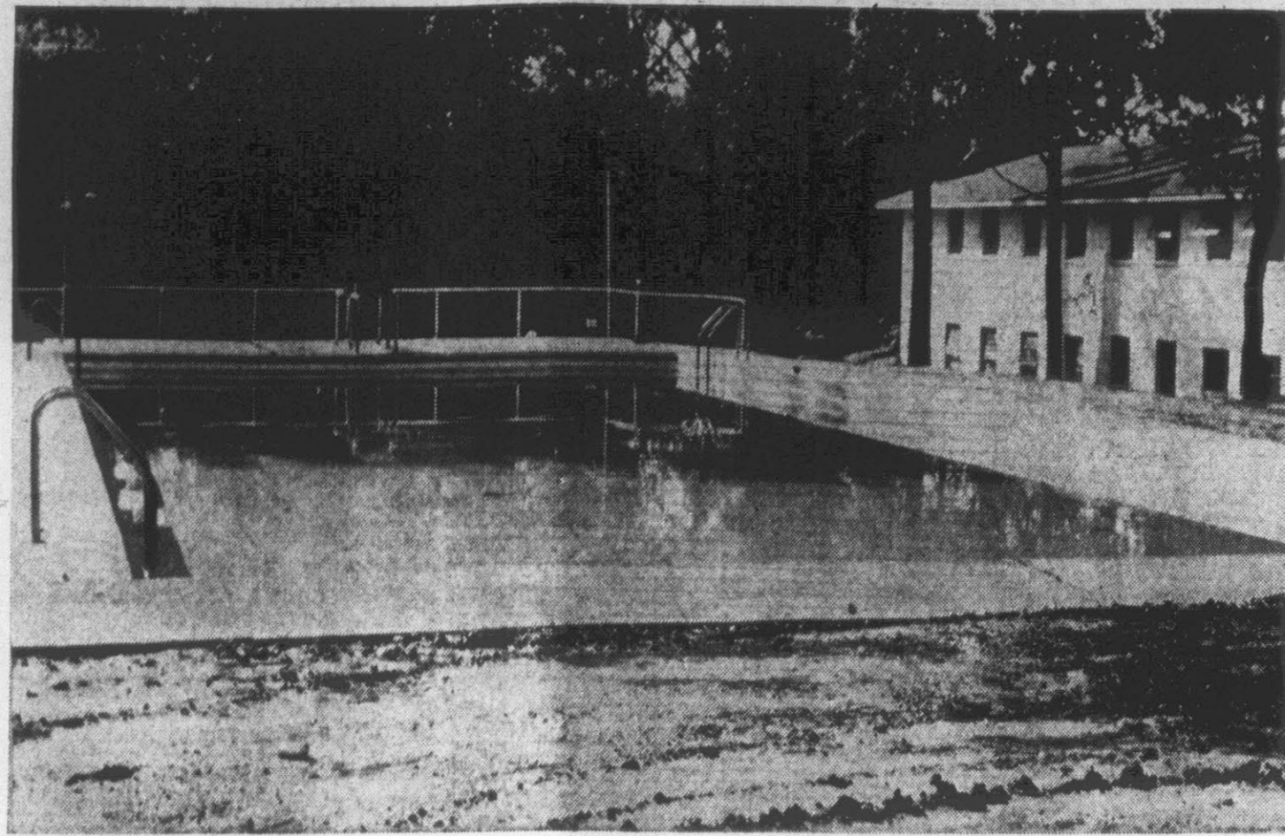
Above is the new $18,000 swimming pool at the Greenville Country Club which is now nearing completion. The pool measures 30 feet by 90 feet. Depth of the pool varies from three feet to nine and one-half feet. In addition, a 20 by 20 foot wading pool has been constructed at the Country Club. Also being built are locker rooms containing 200 lockers and costing about $15,000. (Reflector photo by Alvin Taylor)
