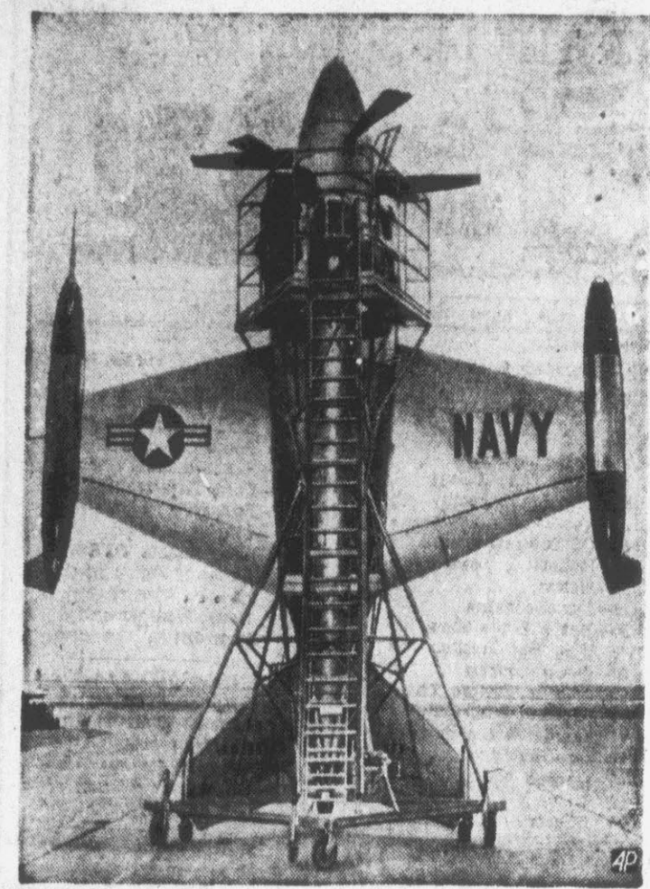
VERTICAL FLIGHT—The XFV-1 vertical rising fighter, perched on its X-shaped tail, is inspected at Edwards Air Force Base, Calif., where it is undergoing pre-flight tests. The plane is raised to vertical position with a special cart—and another platform reached by ladder is used to permit access to the pilot's compartment. The jet craft, built by Lockheed for the Navy, has made only tests in horizontal position so far. The contra-rotation propellers are powered by twin jet turbines. (AP Wirephoto)
