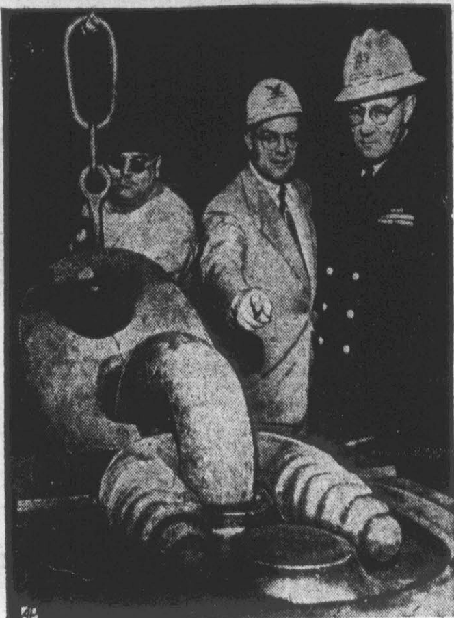
FOR AIRCRAFT CARRIER —One of largest and strongest chains ever made, with 360-pound links, is forged at Boston Naval Shipyard for USS Forrestal. It is 1,800 feet long.
