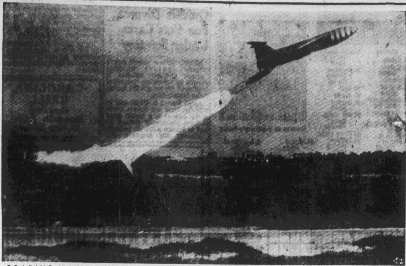
SOARING MATADOR — Air Force B-61 Matador pilotless bomber soars from launcher at Air Force missile test center in Cocoa, Fla. Launcher is mobile and Matador becomes airborne with firing of rocket. Turbo-jet engine takes over once missile is airborne.
