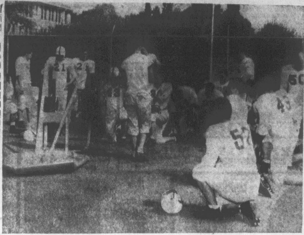
Approximately 30 East Carolina linemen have been hard at work under the tutelage of Jim Mallory, former East Carolina coach and now line coach at East Carolina. Mallory has had the boys practicing tackles and blocks during the first few workouts. (Reflector photo by Tommie Lupton)
