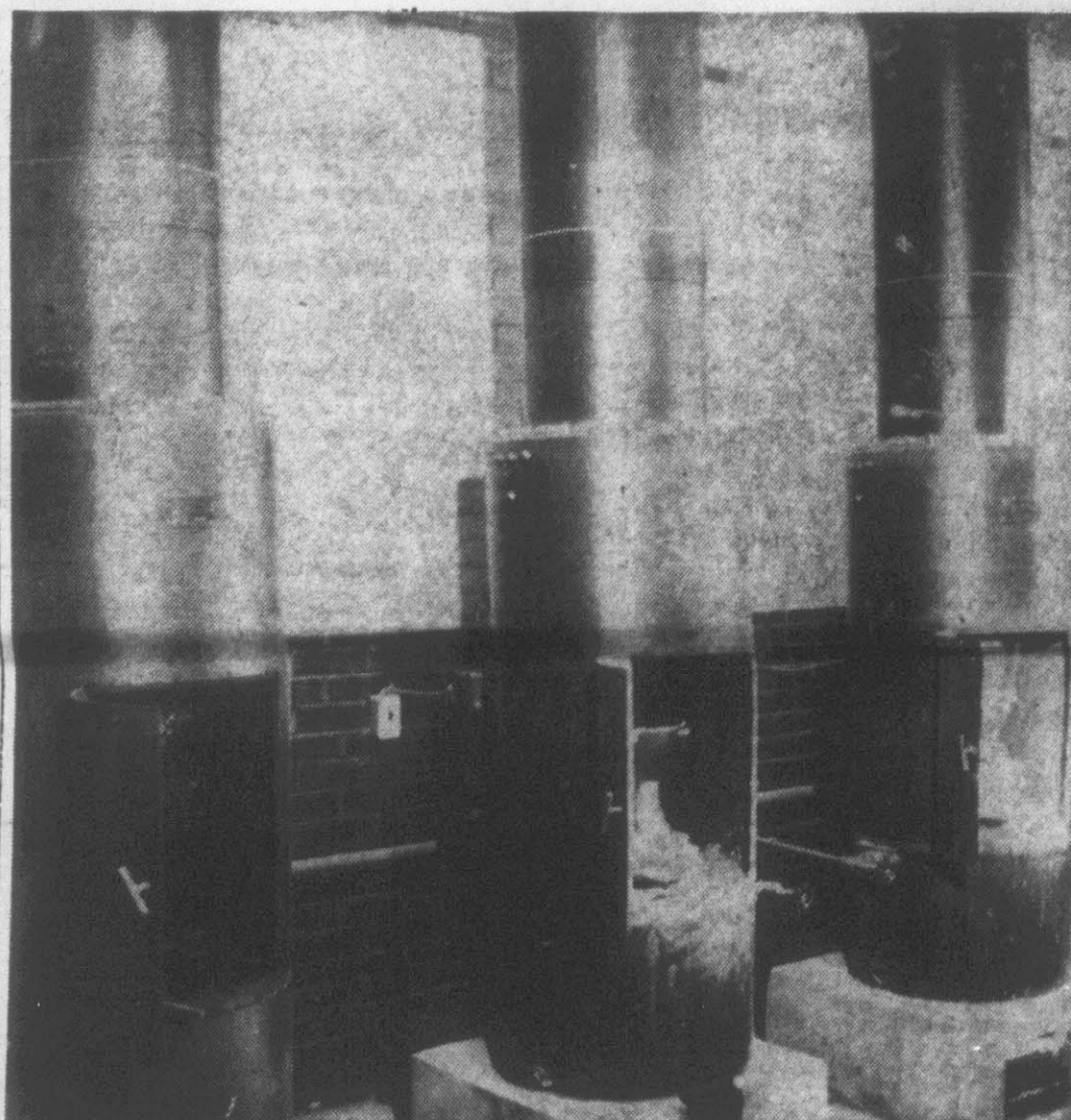
FEED SOURCE FOR MIXING — Here are the 'feeders' which send the proper quantities of alum, lime and vegetable charcoal into the mixing chambers in the early stages of the purifying operation. This mixing takes place in continuous movement after the "raw" water has been brought in from the river.
