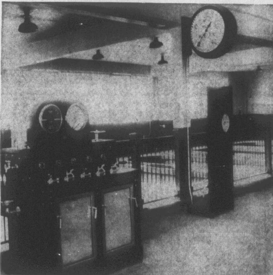
CONTROLS FOR FILTERS — Here is where the valves for opening and closing valves to the filters are regulated, aided by the gauges mounted on top. A separate control lever operates valves for each of the four filters. Just behind the rail are the clear water flumes shown in another picture.
