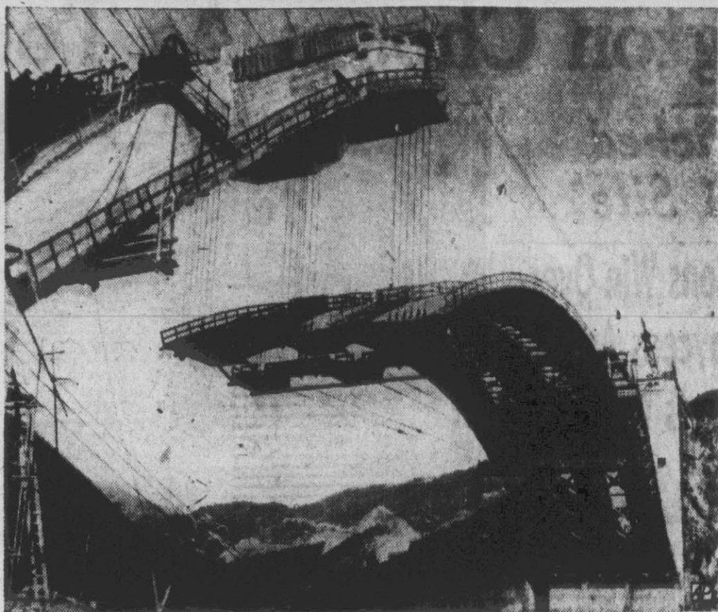
ENGINEERING FEAT — Huge center section of pre-stressed concrete bridge is hoisted in place on 10½-mile Venezuela highway between Caracas and seaport town of La Guaira.
