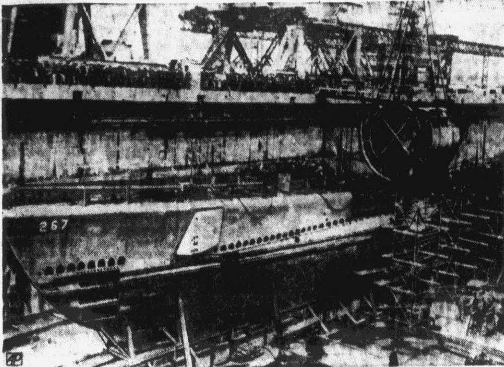
ADDING TO ITS MIGHT—The submarine Pompon lies severed in Philadelphia Navy Yard drydock as workmen lower a new insert with electronic gear into its mid-section.
