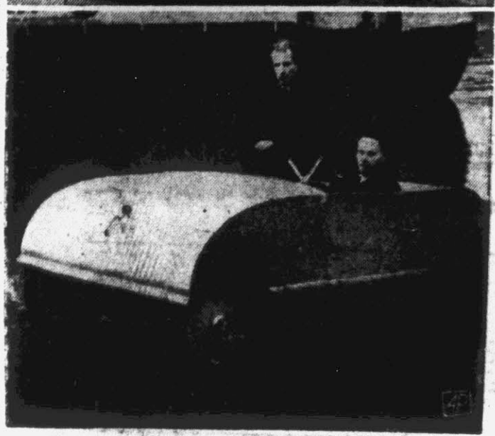
BY LAND OR BY SEA — This vehicle, moves along with ease in water or on land. It's a new amphibious car developed by Karl Baier of Berlin. Baier, shown at the wheel, has simplified construction so that motor, steering system, gear case, clutch, all cables and even the brakes are inside the body. It's possible to drive or sail without any prior changes. The overhead sail is to keep off the sun-light. (AP Wirephoto.)
