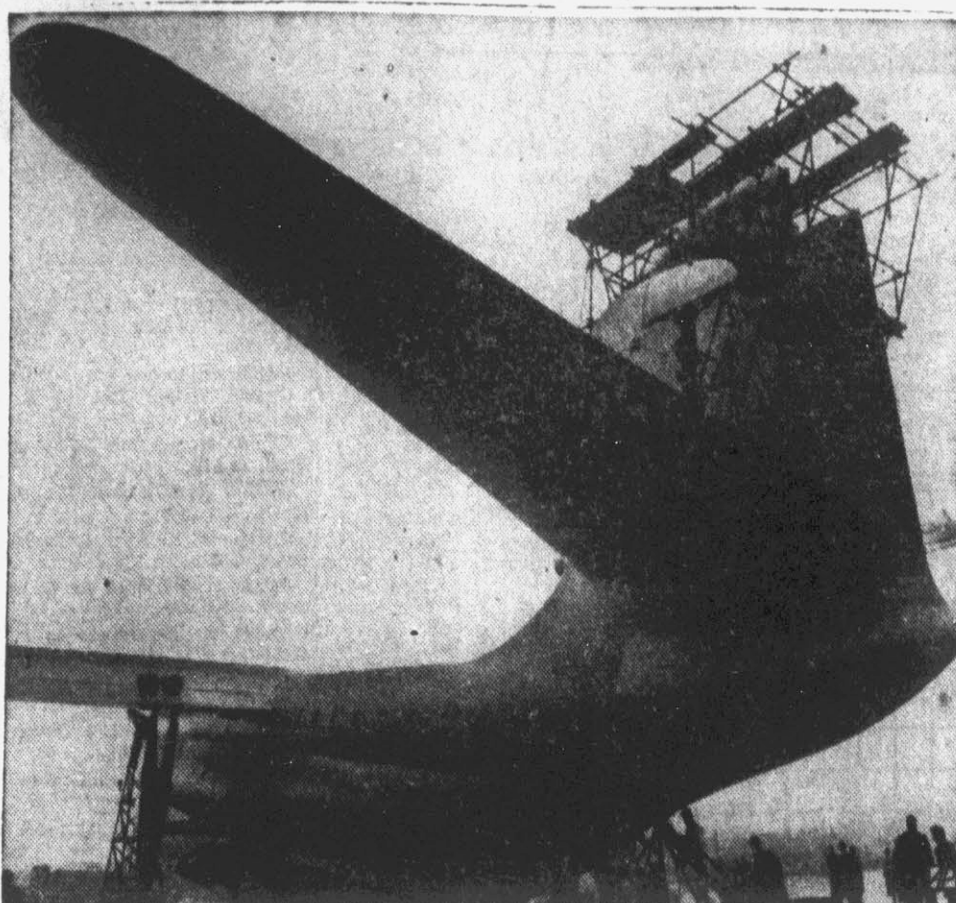
PREPARING TO SOAR—Scaffolding covers giant tall unit of 140-ton British Princess flying boat outside hangar on Isle of Wight. It will carry 200 troops 3,500 miles non-stop.
