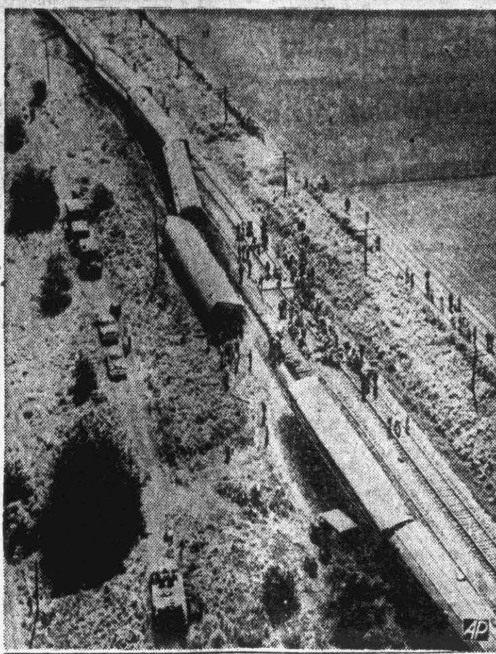
Twenty-six persons were injured in this derailment of the New York Central Railroad's Knickerbocker passenger train near Muncie, Ind. Eleven cars jumped the rails and one turned over. A railroad spokesman said the wreck was caused by a wheel breaking on the Diesel locomotive. The train was en route from New York to St. Louis.—(AP Wire Photo.)
