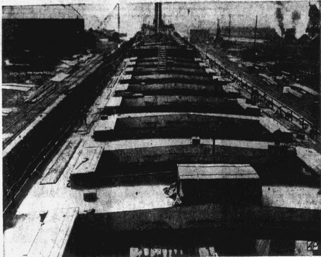
SHIP UNDERGOES STRETCHING—Iron ore ship Philip D. Block lies in South Chicago drydock during 72-foot lengthening process amidships to increase its carrying capacity.
