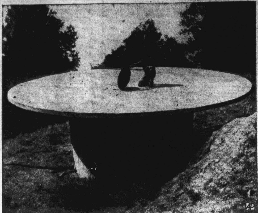
FOREST FIRE TANK —Robert A. Bulkley, Forestry Service engineer, inspects one of 53 concrete basins, each holding 5,000 gallons of water to fight forest fires near Pasadena, Cal.
