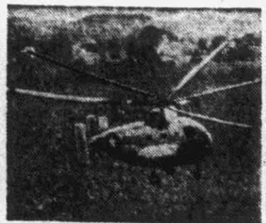
AP Newsfeatures KELETT KH-10, a twin-engined transport-type Air Force helicopter, is all-metal, has a cruising speed of 80 miles per hour, cruising range of 350 miles. It can carry 12 men.
