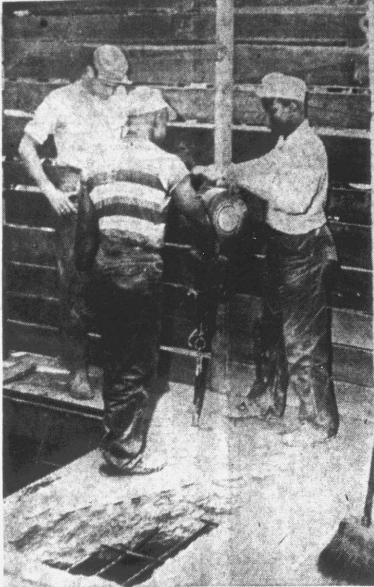
Workers of the R. H. Boulligny Company, Inc., of Charlotte are pictured here as they break the cement covering over the Fourth Street sub-station, which is to be enlarged and new equipment placed there. The present sub-stations located on fourth street have three small units which are unable to take care of the up-town load. New transformers arriving in Greenville Monday will be installed in each of the sub-stations. (Reflector Staff Photo by Roy Hardee.)
