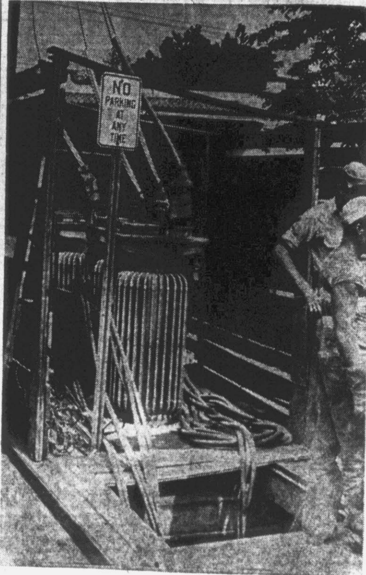
Temporary transformers are in the above picture taken at the Fourth Street sub-station this morning. The sub-station is being enlarged to take care of new and larger transformers to be installed there next week. The unit will help ease the overloaded condition of the uptown business section in the summer months. (Reflector Staff Photo by Roy Hardee).
