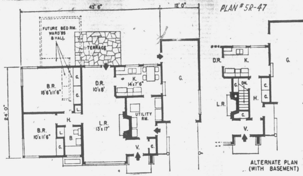
AP Newsfeatures A FLEXIBLE PLAN for use with or without basement, this is design 5R-47 by Elmer Gylleck, Architect, 120 So. Grove Ave., Elgin, Ill. It can be used for two or three bedrooms, an expandable feature that needs no excess attic construction. Without basement, the house comprises 16,600 cubicfeet including garage. A basement brings this up to 19,500. Local builders know the average cost per cubic foot for this type of house. The architect suggests an exterior of wood siding and stone dressing with a roof of wood or asphalt shingles.
