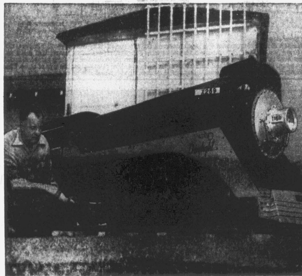
FRUIT OF A HOBBY—Mechanic Remels Loon, of South Pasadena, Cal., examines working locomotive of his scale model of a Daylight Streamliner which took him five years to build.
