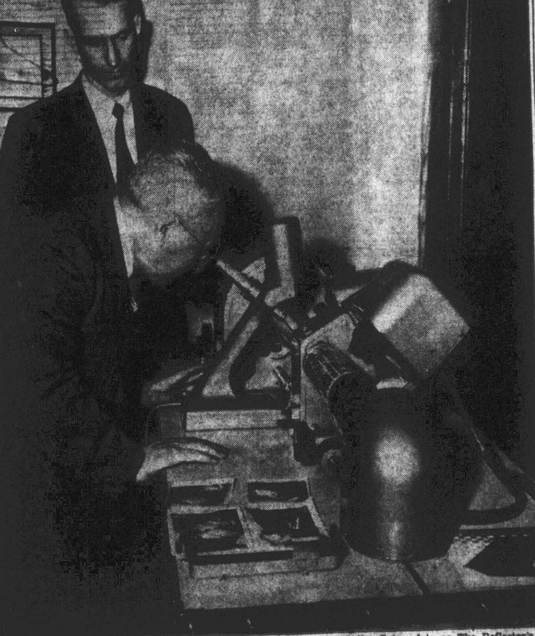
Publisher D. J. Whitchard, Jr. takes a look through the stroboscope at the flying dots as The Reflector's newly installed Fairchild Electric Photo Engraver transfers the images of the photographs on the right cylinder to a plastic plate on the cylinder to the left. The red hot cutting stylus doing the actual cutting operates at 240 vibrations per second and covers a one by eight inch surface every three minutes. Looking on is W. F. Rudder, Fairchild expert who completed installation of this modern piece of equipment for The Reflector yesterday.
