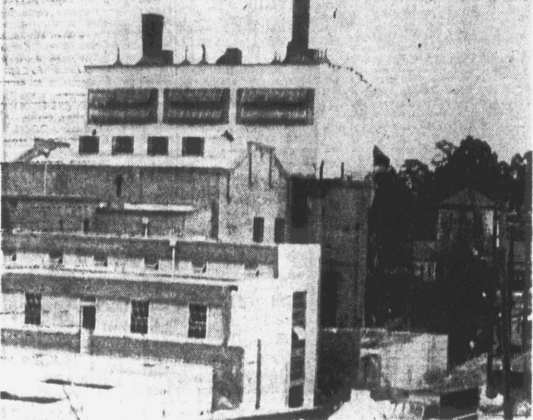
The overall shot of the Water and Light plant shows the entire plant and the section which is being erected to house a new 5,000 kw turbine generator.
