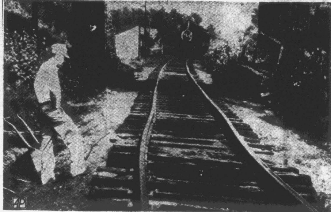
A prolonged heat wave has caused buckling of these rails on Central Branch of the Boston & Maine railroad near Hudson, Mass. The track is out of line nearly five inches. Traffic over the line was delayed for two and a half hours for repairs. Seven deaths from the heat throughout New England were reported Thursday. (AP Wirephoto).
