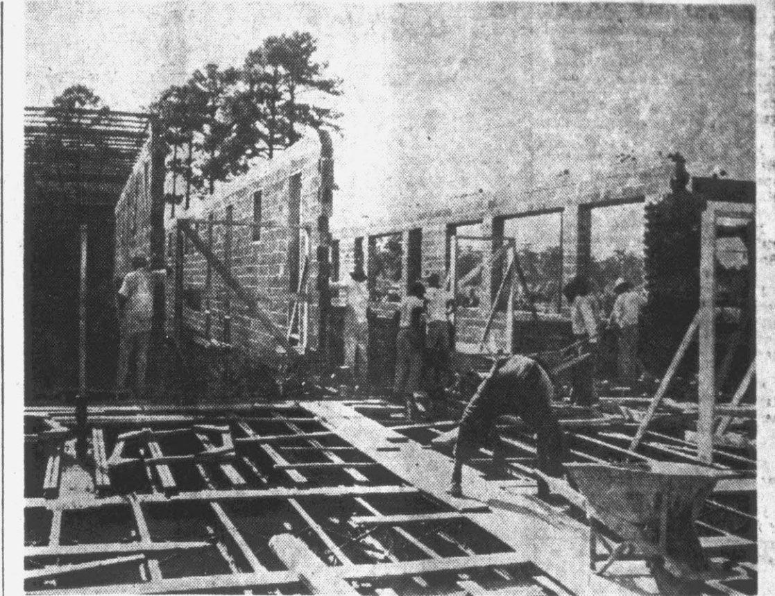
Workmen lay bricks and concrete blocks in the wall of the $165,000 fire-resistant school building at Farmville which will house the Negro elementary and high school students. The building is the largest constructed in the county school system since the Ayden school was built in 1930. It will have 18 class rooms, offices, and a teachers room. An auditorium and lunchroom are to be added to the building when funds are available. (Daily Reflector photo)
