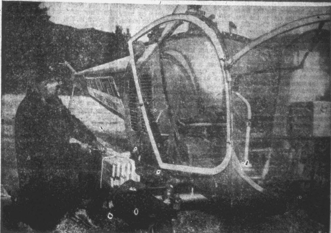
OPERATION WINDMILL —Materials for a fire lookout tower on top of 3,260-foot Mt. Pequawket, near Kearsarge, N. H., are ferried in by helicopter. Top: Pilot Edwin Packer hovers over the area. Bottom: Everett Ward of Bartlett, N. H., secures lumber on side of machine. Project in less than 2 weeks saves labor of estimated 15 men back-packing load over 5-week period.
