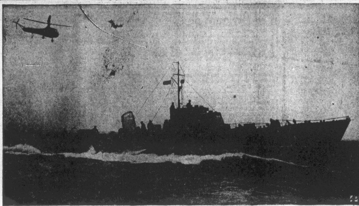
'JET' WARSHIP TRIED OUT—A British "jet" motor-gunboat makes speed run while observation helicopter flies overhead. Craft is powered by an improved gas turbine engine which has many features of the aircraft jet engine, although power still is transmitted to an orthodox propeller. Trials will include running engine for 400 hours under sea conditions.
