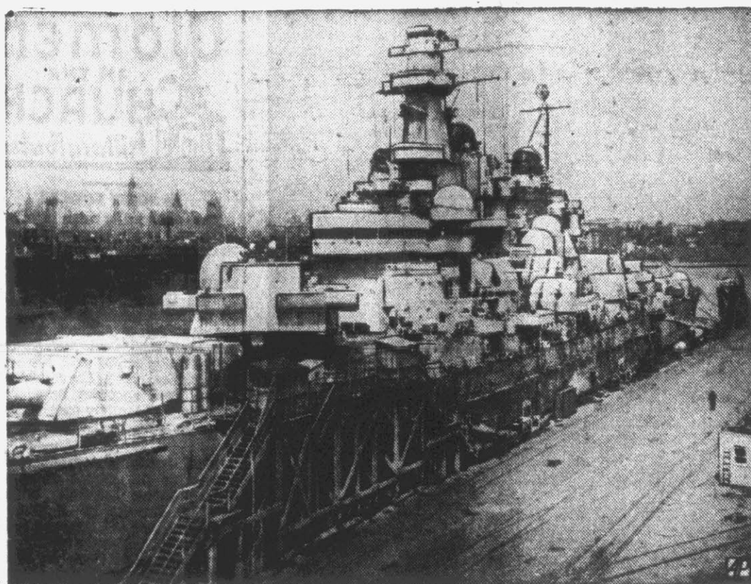
PRESERVING BATTLEWAGON —The 45,000-ton battleship New Jersey undergoes preservation job at the Naval Shipyard in Brooklyn before being laid up at Bayonne, N. J.
