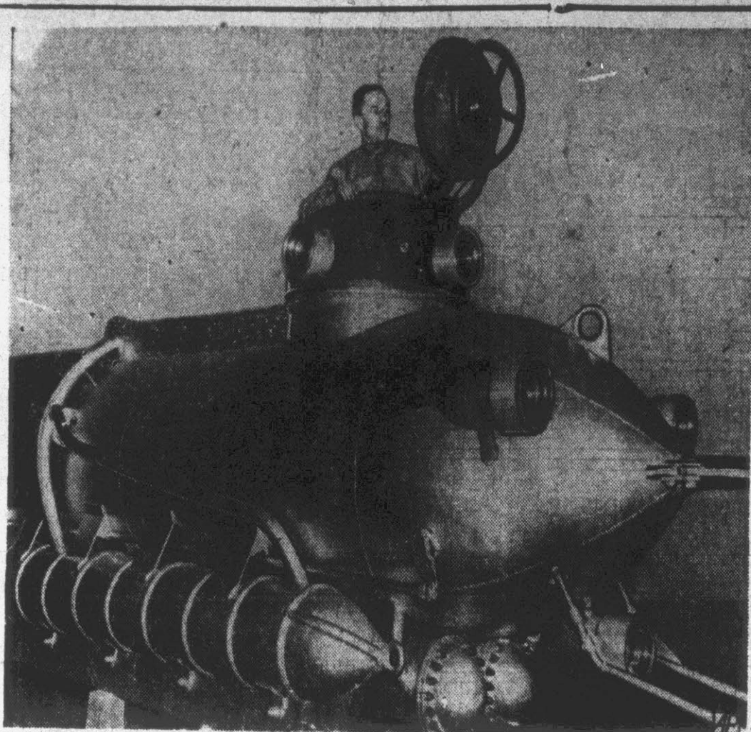
NEW ITALIAN SUBMARINE —Pietro Vassena stands in conning tower of midge submarine he invented at his home at Lake Lecco, Italy. The craft, 25 feet long and 4 feet, 6 inches wide, was designed for scientific work and retrieving treasure from sunken vessels. Prof. Auguste Piccard, explorer of the stratosphere, will aid in testing the craft.
