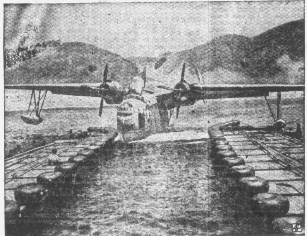
MOBILE SEAPLANE SLIP —A U. S. Navy flying boat eases into a new, self-propelled seaplane berth developed by the Navy. It is built of pontoons and operates along a 600-foot submerged cable. Water jets push plane from side to side as desired.
