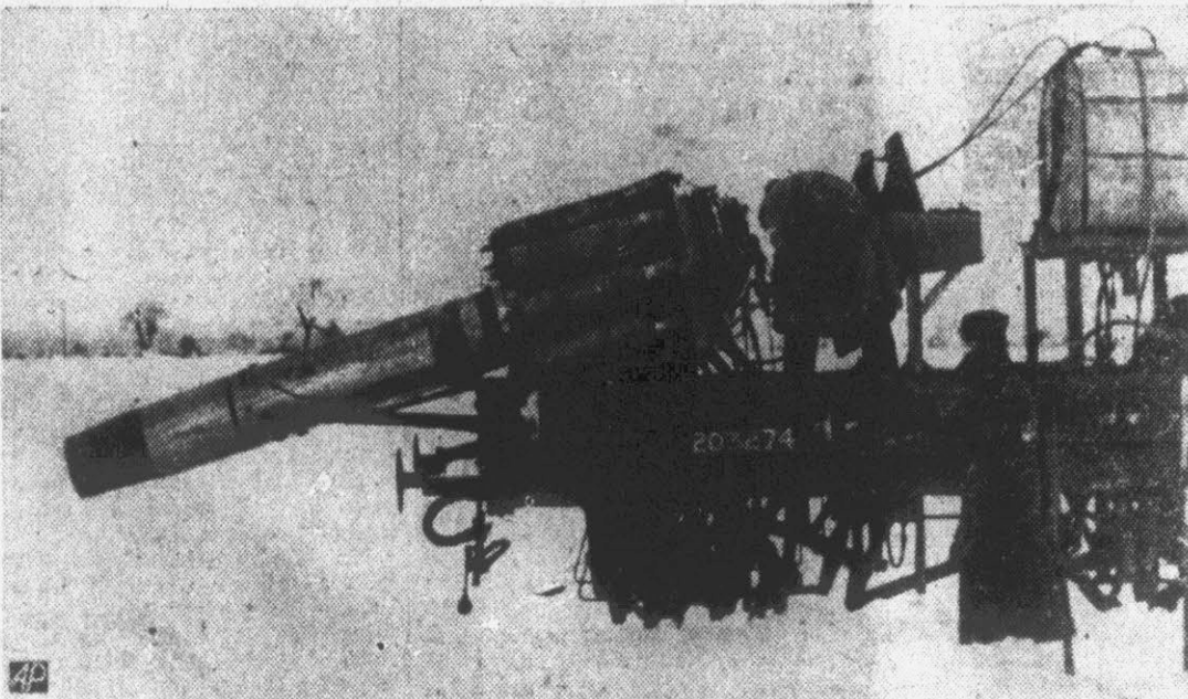
JET SNOW SHOVEL —An aircraft gas turbine engine, mounted on a railway car, is used to melt and blow away snowdrifts on tracks near Grantham, England.
