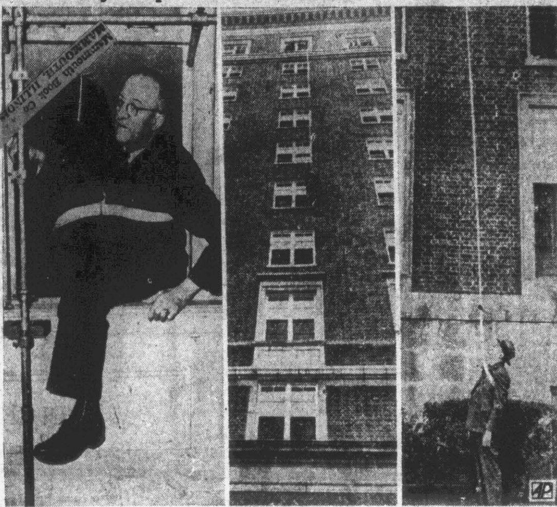
John Bassett, 65-year-old barber from Detroit, demonstrates his "Safety-Scape" at a hotel in Atlanta, Ga., for firemen and underwriters. Designed to save persons trapped in hotel fires, the simple mechanical device permits descent by a steel ribbon released from an automatic reel. Left: Bassett leaves a 12th story window of the hotel with a strap looped under his arms. Center: He descends at elevator speed. Right: Safely on the ground, he has completed the 12-story drop in about 18 seconds. (AP Photos).
