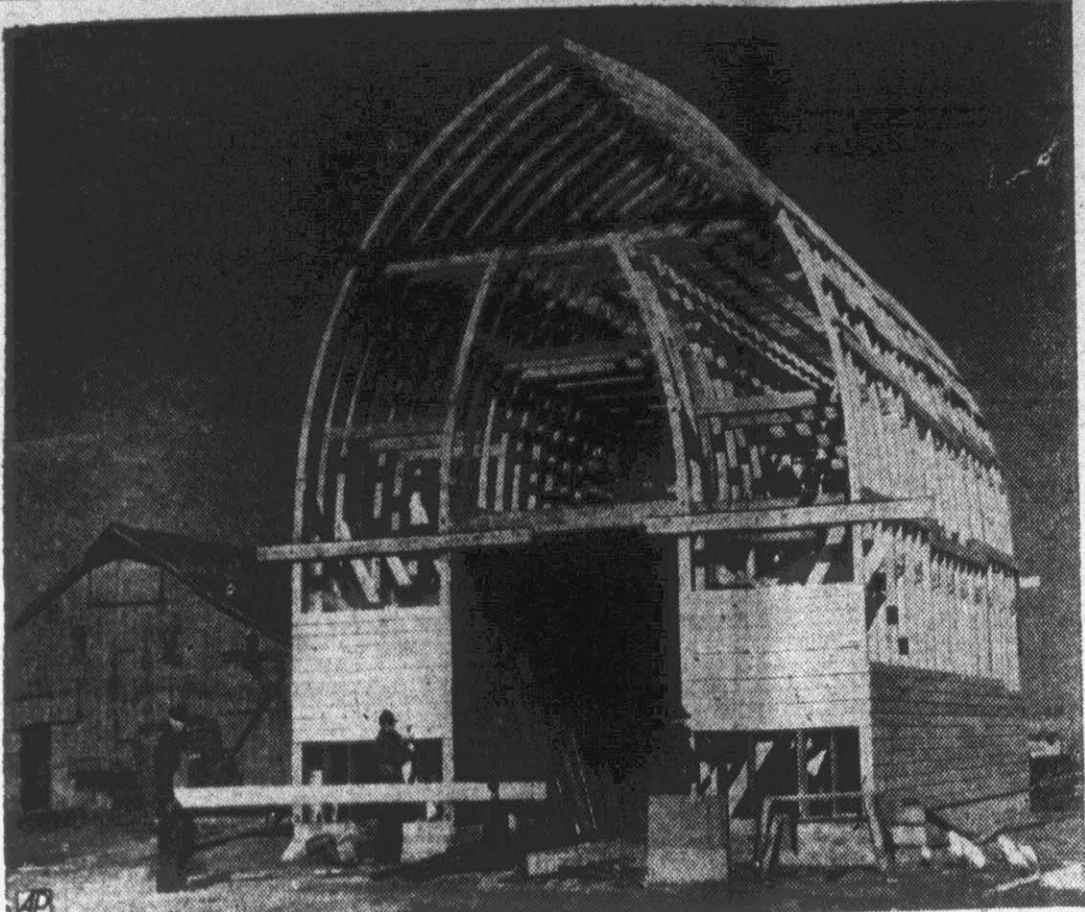
BIG CORNCRIB — Workmen put up a mammoth pre-fabricated crib near Decatur, Ill. The crib has a capacity of 5,500 bushels of ear corn plus an overhead granary holding 2,700 bushels of small grain. The framework comes pre-cut and is bolted together.
