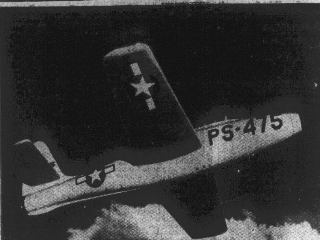
THUNDERJET IN FLIGHT —The Army's new P-84 jet fighter plane, the Republic Thunderjet, roars through the clouds on a test flight. It has been timed unofficially at 619 miles per hour, has a wing span of 36 feet, 5 inches and an overall length of 37 feet. In contrast to other American jets, the P-84's air intake is in the nose instead of on the sides.
