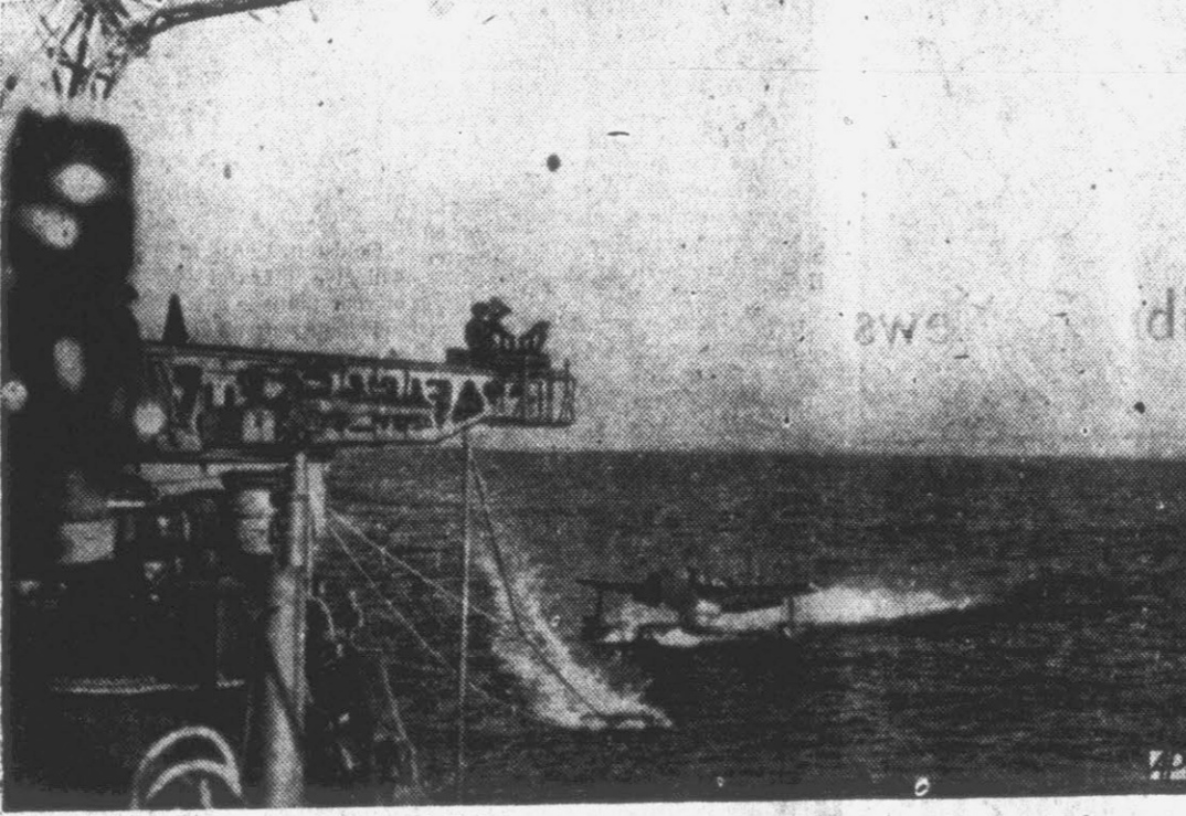
PLANE TAXIS TO SLED —In a Navy demonstration showing how scout planes are recovered, this plane taxis to a sled before being hoisted aboard the USS Denver. In this method, a sled is allowed to stream behind the ship; the plane taxis to the sled; the sled is then reeled into position, under a crane waiting to hoist the plane aboard.
