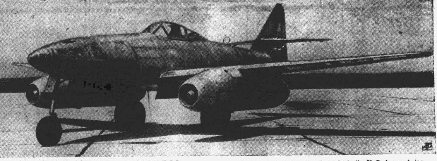
GERMAN JET-PROPELLED FIGHTER—This Messerschmitt 262A-1, first of its type brought to the U. S., is now being studied by engineers of the Air Technical Service Command. Its level flight speed is estimated from 515 to 530 mph.
