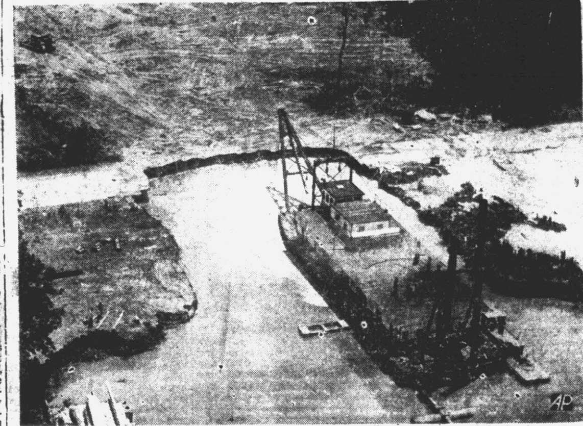
After pumping out all of the sand within reach in the Pasquotank river near Elizabeth City to supply a million cubic yards of fill for the new causeway across the swamp, a big dredge of the R. C. Huffman Construction Company moves up to take an enormous bite out of Camden county for more filling material. The dredge is cutting its way across the Elizabeth City-Norfolk highway where traffic was suspended for 48 hours while the dredge worked its way forward. After the dredge ate its way into the clearing (background), a pontoon bridge (lower left) was swung into place on the highway. (AP Photo).
