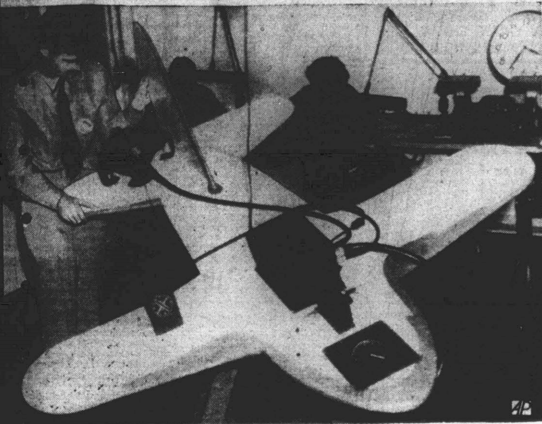
Lieut. (JG) T. A. Johnston of Livingston, Ala., demonstrates at Philadelphia, Pa., the operation of a type of compass, described by Bendix Aviation Corporation as enabling pilots to "put the finger" on their objectives and to return home unerringly. Known as the gyro flux gate compass, it uses the magnetic field in its operation. (AP Wirephoto).
