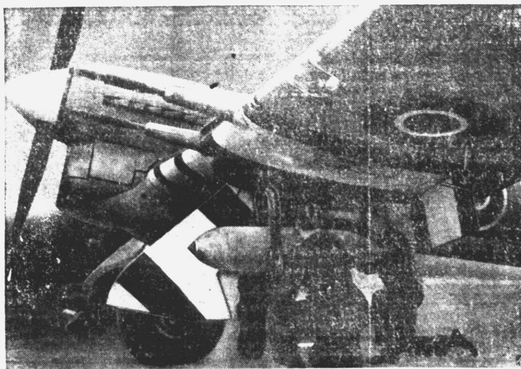
BOMBS FOR TYPHOONS — The RAF's fast Typhoon fighter now can carry two 500-pound bombs, one of which is shown being fitted to the plane. Note 20-mm. cannon in wing.
