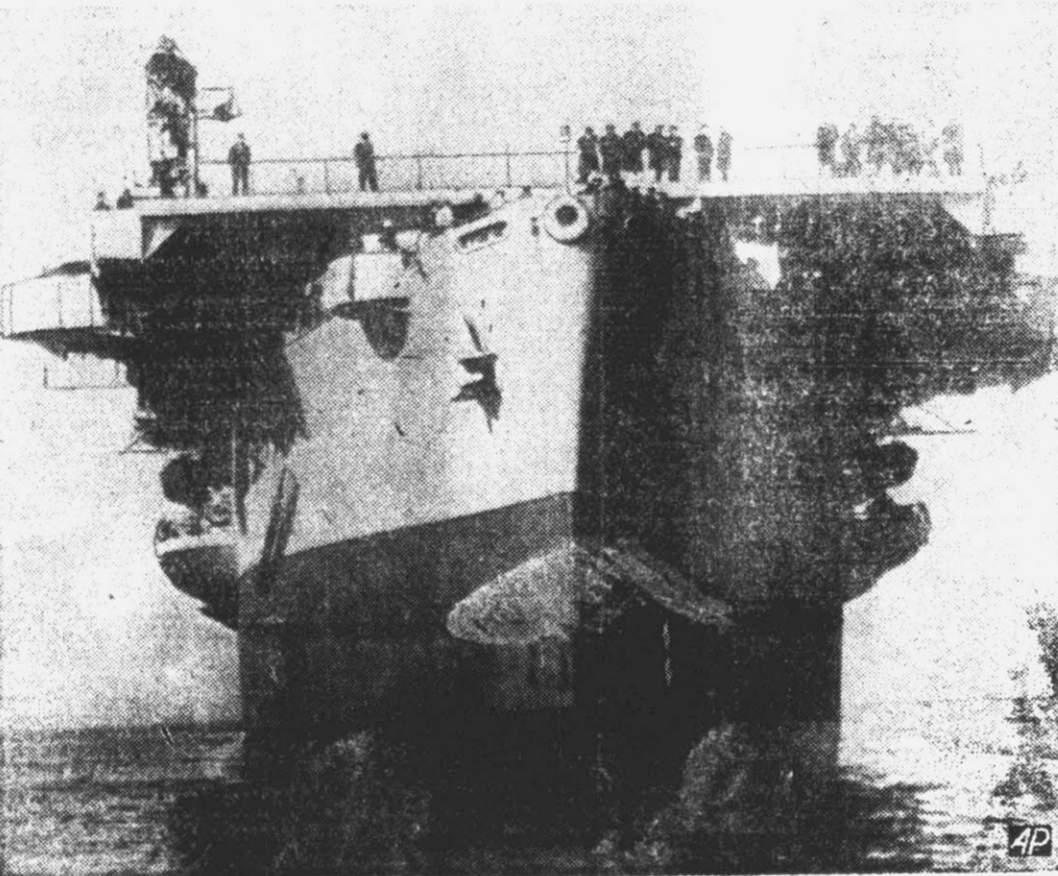
The U. S. S. Breton, a new type of speedy aircraft carrier, rests in the water at Tacoma, Wash., following her launching three weeks from the time her keel was laid.
