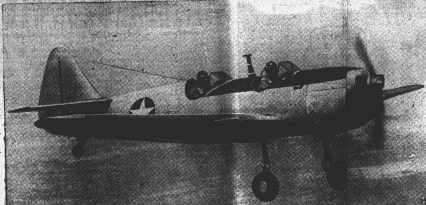
IT'S PLYWOOD —This new Ryan PT-25 military primary training plane is made of plastic-bonded plywood. Aluminum alloys and all strategic materials have been eliminated except for engine cowling which is 2 per cent plane's weight.
