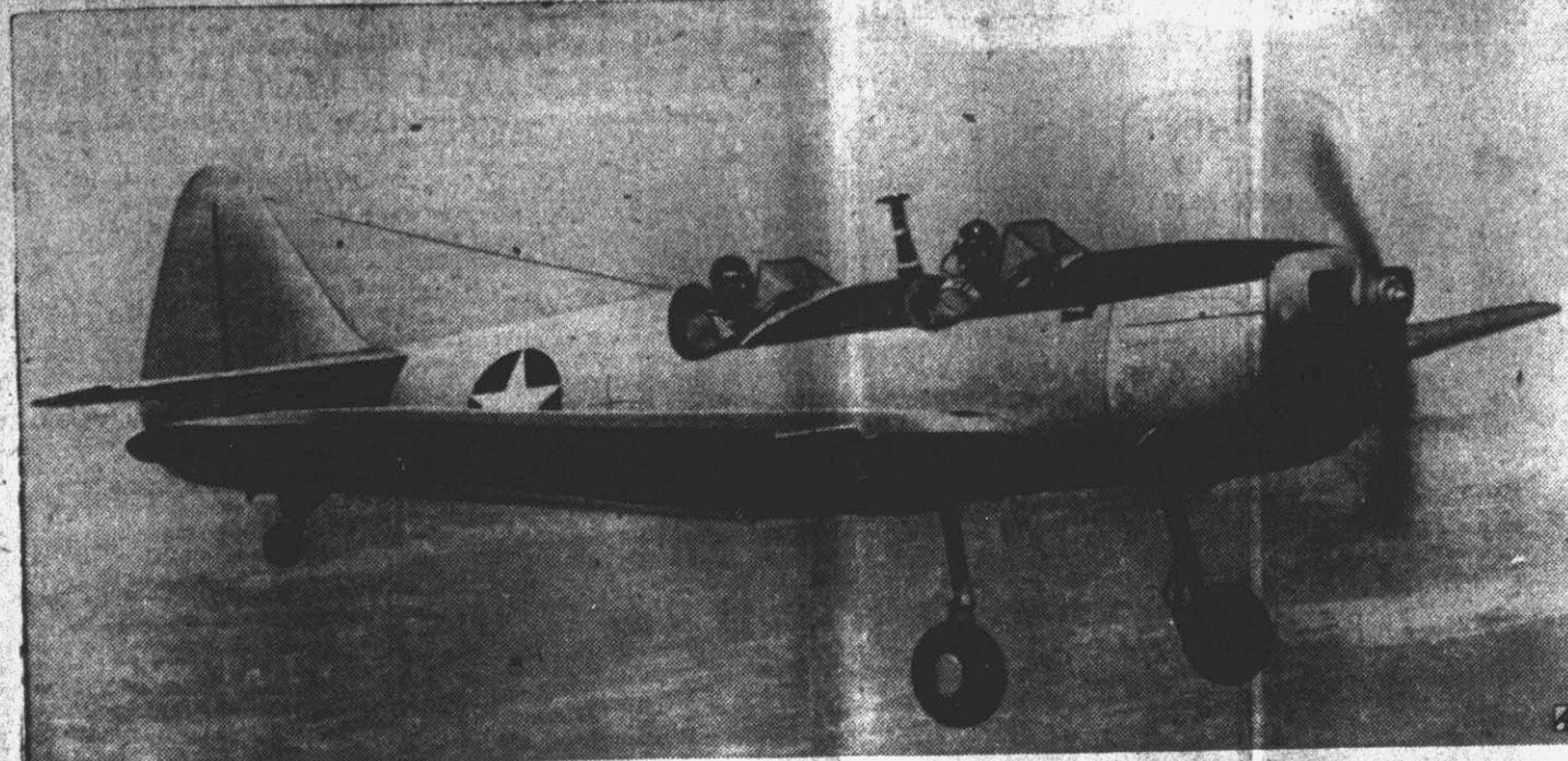
IT'S PLYWOOD —This new Ryan PT-25 military primary training plane is made of plastic-bonded plywood. Aluminum alloys and all strategic materials have been eliminated except for engine cowling which is 2 per cent of plane's weight.
