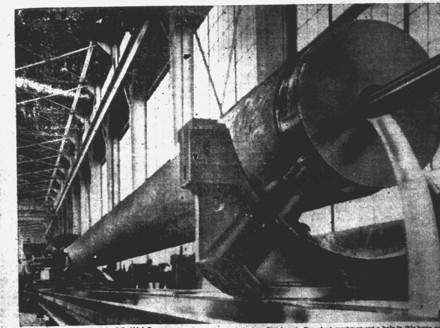
FORGING A TOOL OF WAR—Using an 84-inch boring lathe in a Pittsburgh, Pa., plant, workmen cut a hole in this huge gun forging nearly 70 feet in length. This giant piece of machine work is typical of heavy industrial war production in Pittsburgh area.
