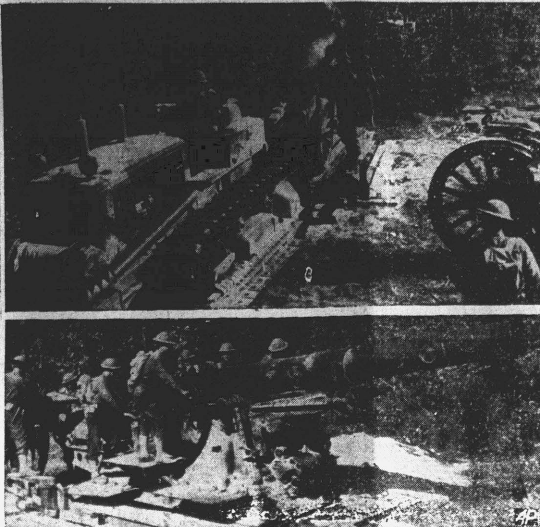
Twelve of these big 240 mm. howitzers, biggest field guns in the army, are ready for action during army maneuvers in the vicinity of Hoffman, N. C. Top: A 10-ton Diesel-engine tractor teams up with another tractor to haul the big gun into position. Bottom: The field piece is set up and ready which means hurling a 345-pound projectile as high as five miles into the air. In accuracy, it is said to compare with a rifleman hitting the bull's eye at 1,000 yards, its probable error for range being 25 yards—beyond or in front of its target—at 14,000 yards.
