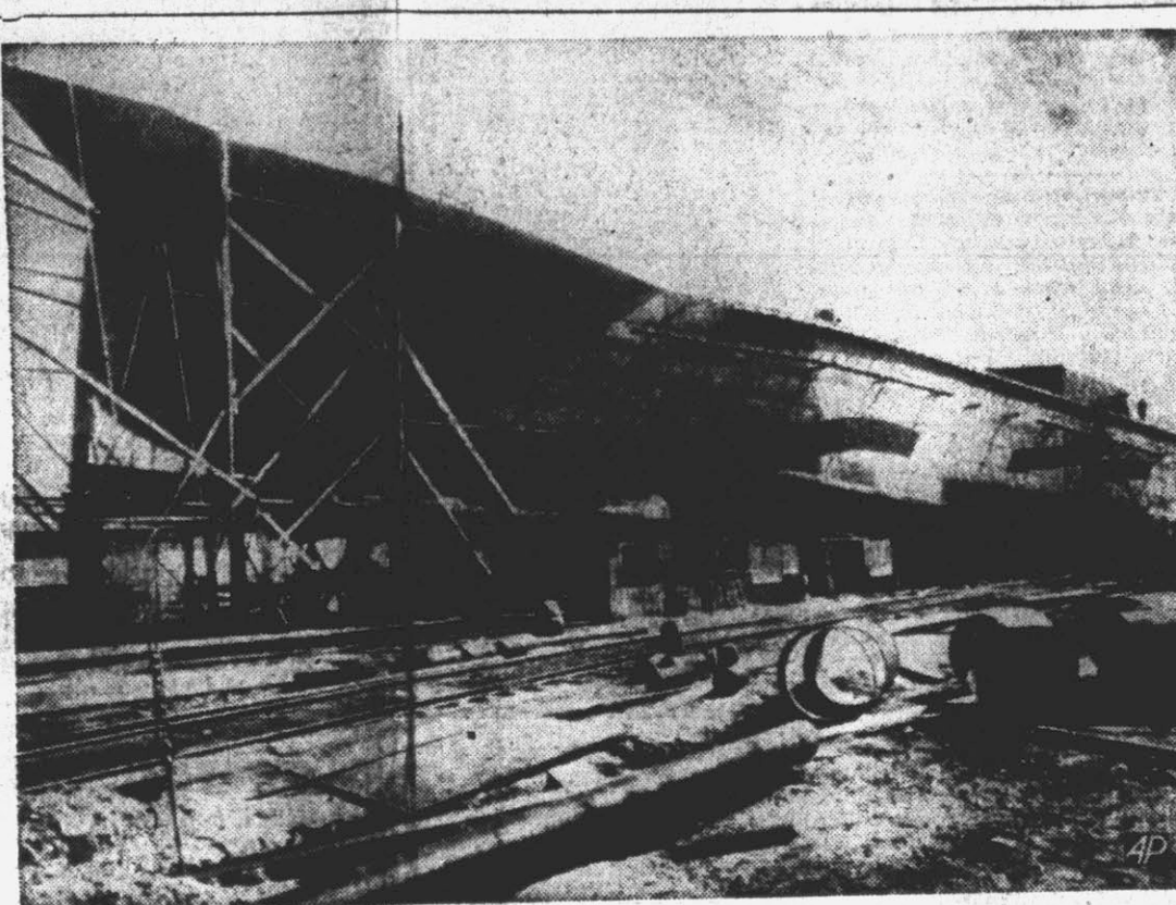
The "Sea Otter," first of a new type cargo ship of revolutionary design which the navy regards as a challenge to submarine warfare, is shown in this official navy photograph under construction at the Levington Shipbuilding company's yards at Orange, Texas. Light in weight and with propeller amidships, such vessels could be turned out in two months' building time, in the opinion of navy engineers.
