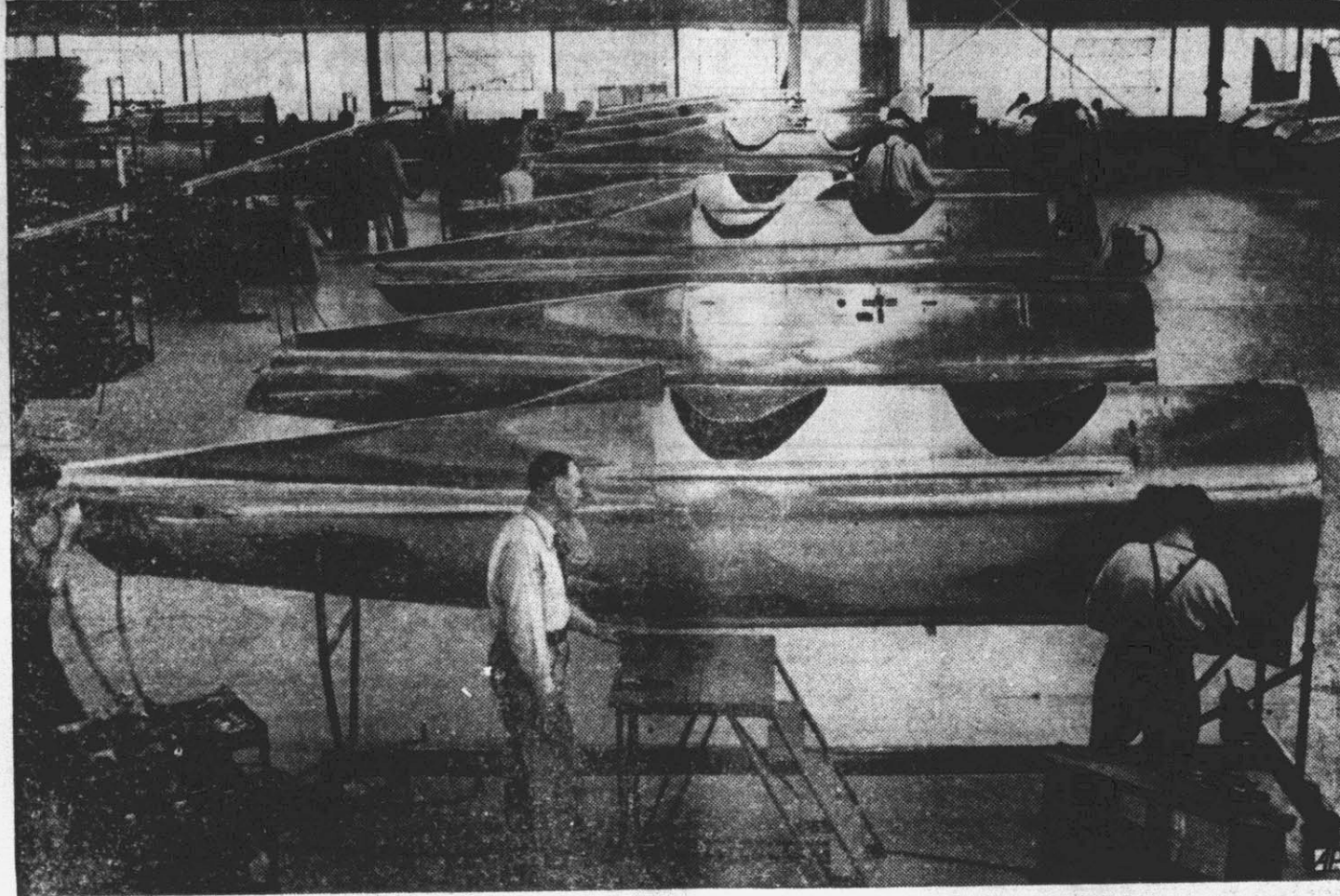
TURN THE CONES DOWN ON THEIR SIDES —Stretched out, the conical riveted sheets of aluminum alloy that the Ryan Aeronautical Corp. plant in San Diego transforms into planes, becomes part of a fuselage. Engine, wheels and wings come next.
